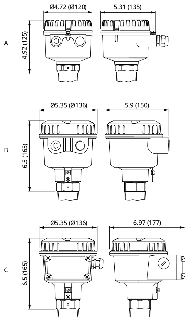
Figure 4: Rosemount 2501 Housing Options
