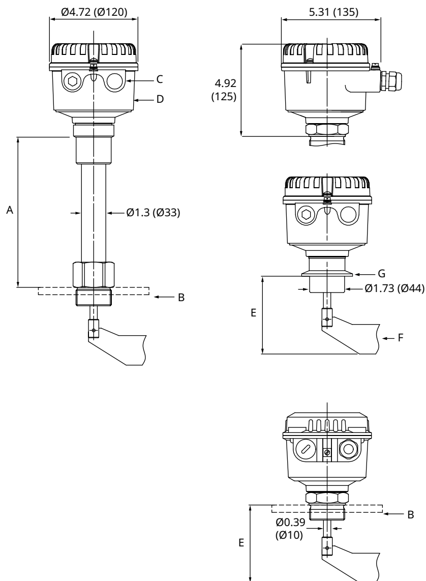
Figure 5: Rosemount 2501 Paddle Level Switch (Standard Length, Application Profile code L)
