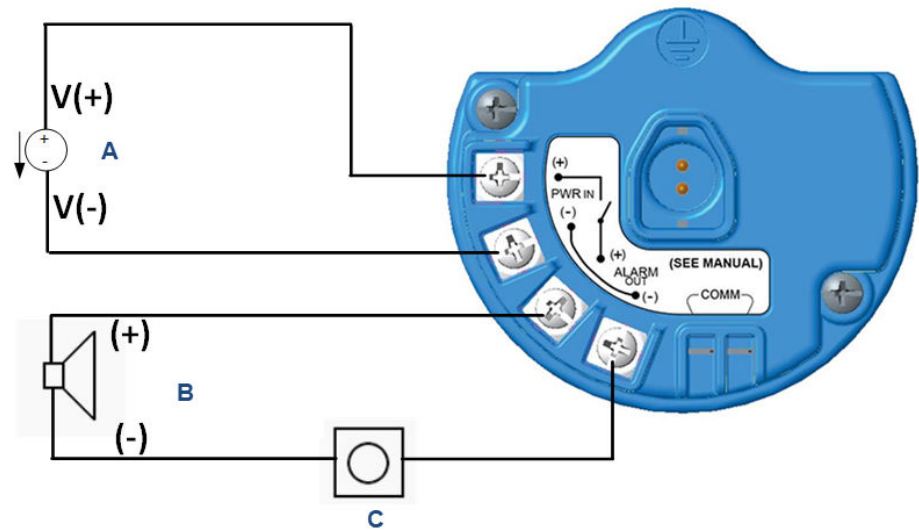
Figure 3-6: Four-Wire Installation
