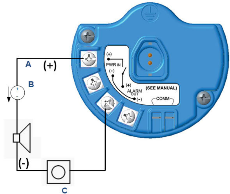
Figure 3-7: Two-Wire Installation
