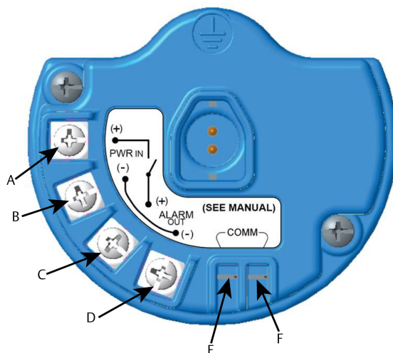
Figure 3-5: Terminal block
