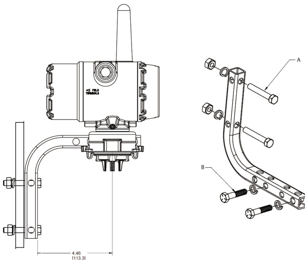
Figure 3-4: Panel Mounting
