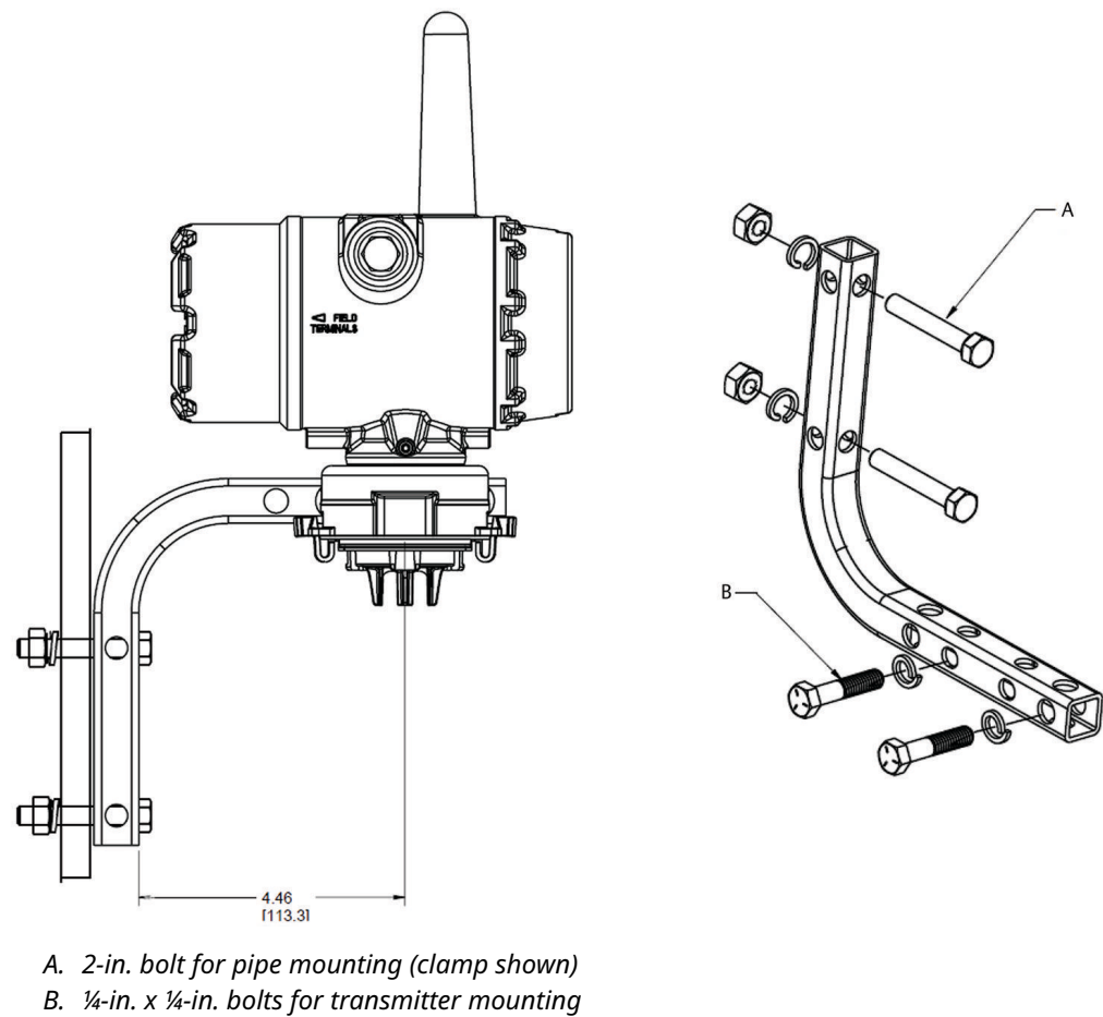
Figure A-2: Rosemount 928 Mounting Configurations
