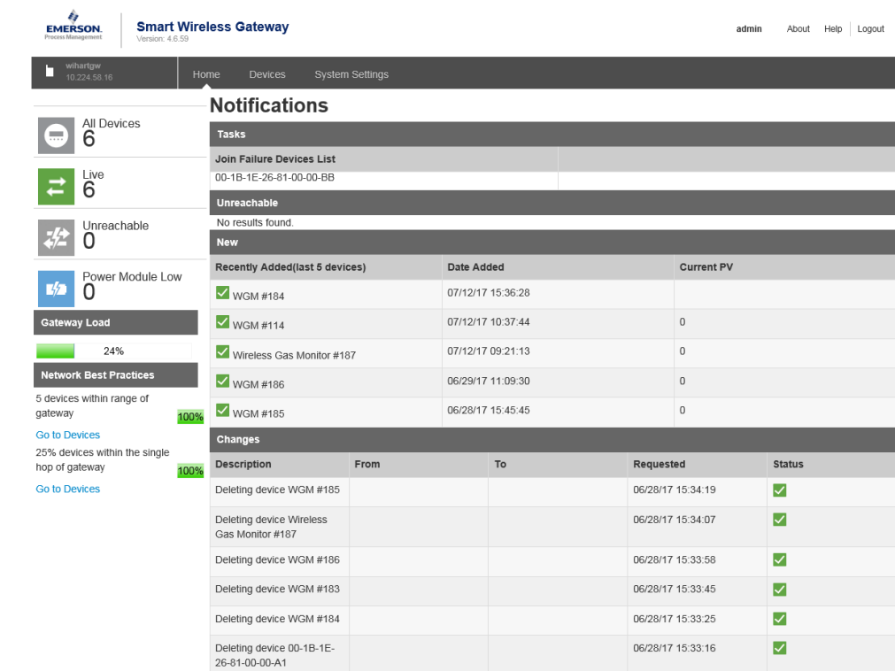
Figure 4-2: Web interface
