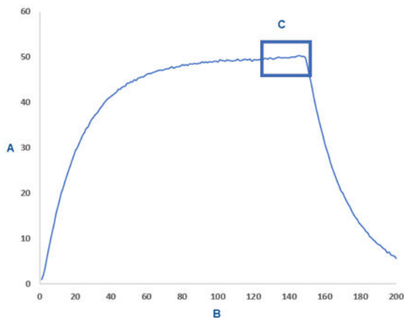
Figure 2-8: Typical calibration profile
