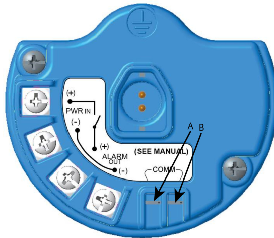
Figure 2-9: HART terminal
