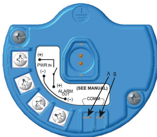
Figure 2-6: Transmitter terminals
